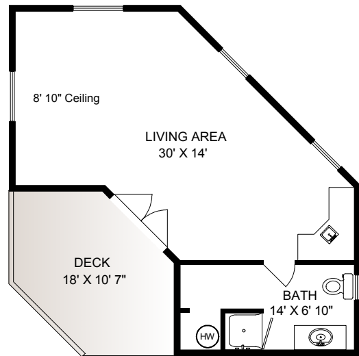
COTTAGE 534 SQ. FT.
