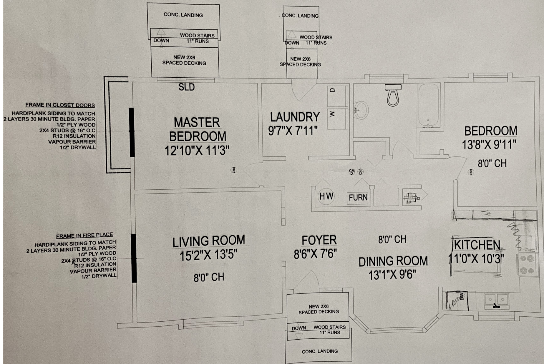
EXISTING FLOOR PLAN 1,175 SQ.FT.
